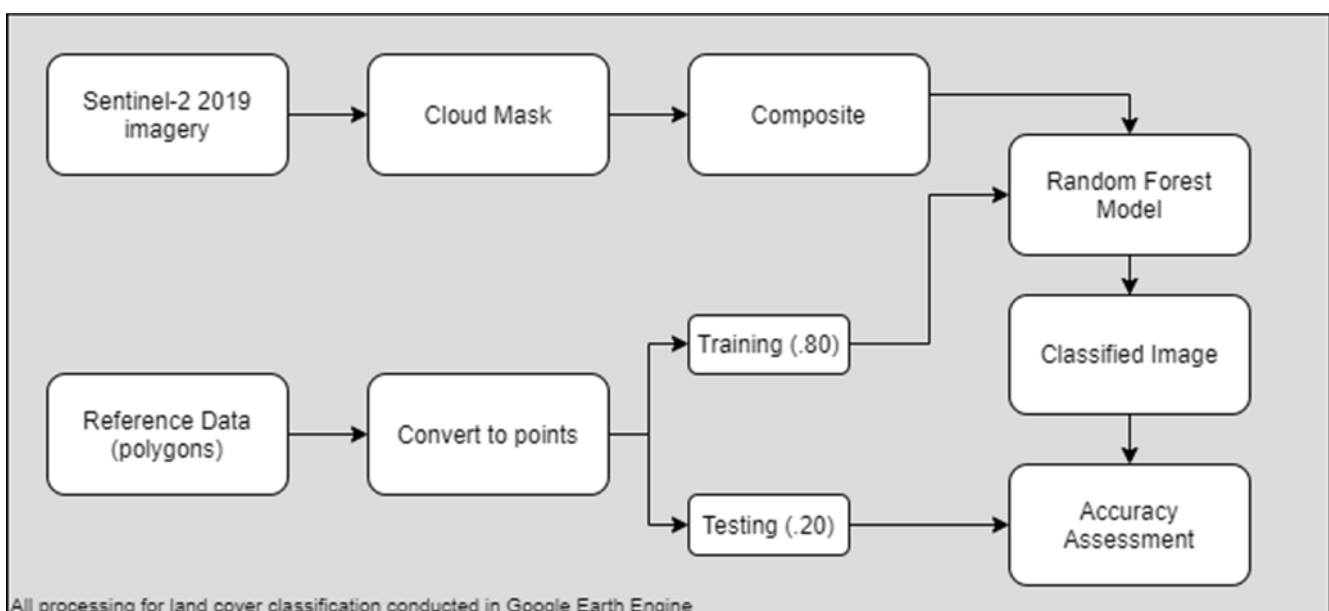
Figure 2. Flowchart showing the workflow used for the land cover classification in Google Earth Engine.
